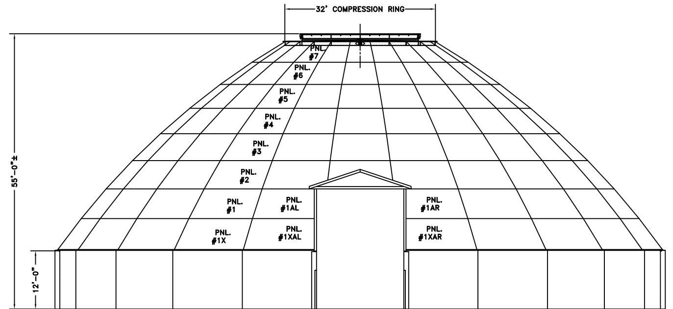
R124 DIA. DOME ON 12' WALL HGT.
